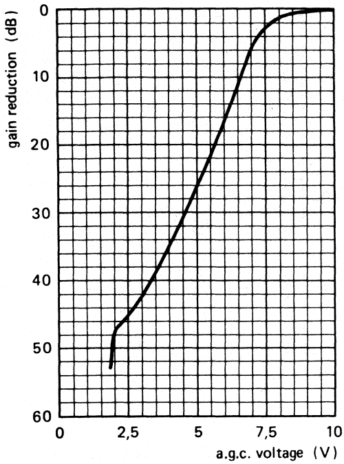
Fig. 4 Typical a.g.c. characteristic, low v.h.f. band.
