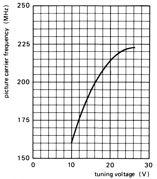
Fig. 8 Typical tuning characteristic, band III.
