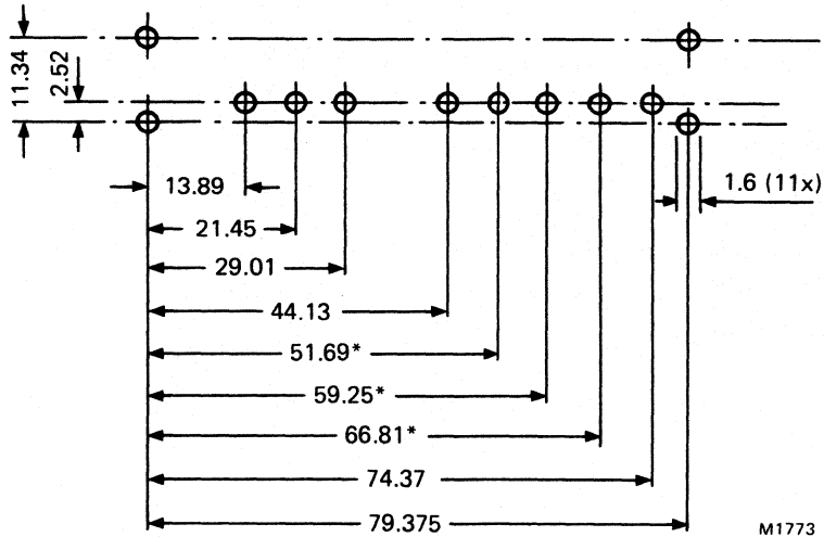
Fig.3 Piercing diagram viewed from solder side of board.
