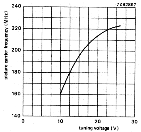
Fig. 8 Typical tuning characteristic, high v.h.f. band.
