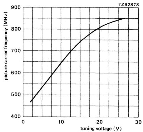
Fig. 7 Typical tuning characteristic, u.h.f. band.
