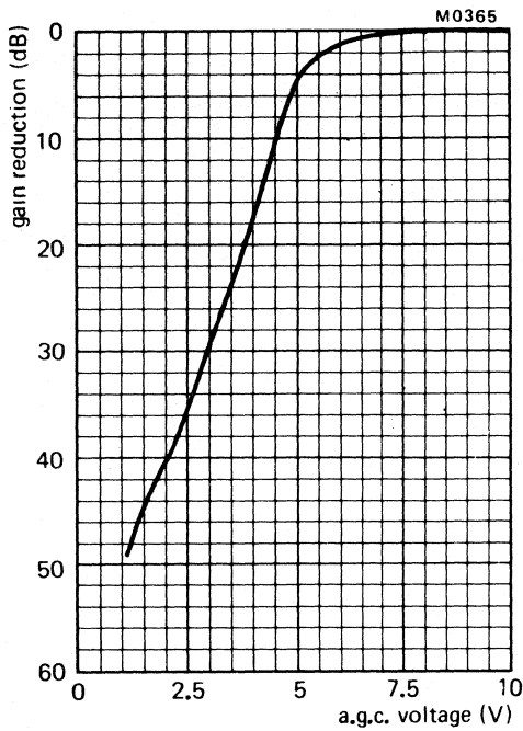
Fig. 3 Typical a.g.c. characteristic, low v.h.f. band.
