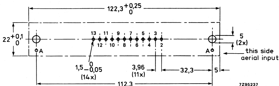
Fig. 3 Piercing diagram viewed from solder side of board.
