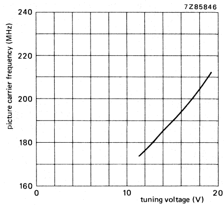
Fig. 5 Typical tuning characteristic, high v.h.f.
