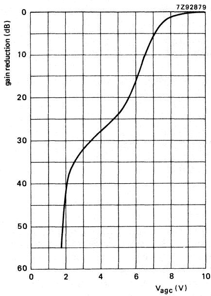
Fig. 4 Typical a.g.c. characteristic, v.h.f. band.
