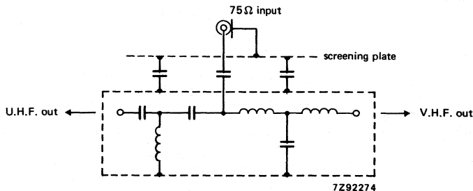
Fig. 1 Electrical diagram.
