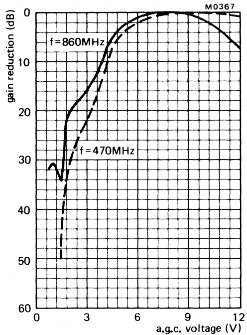
Fig. 6 Typical a.g.c. characteristic, bands IV and V.
